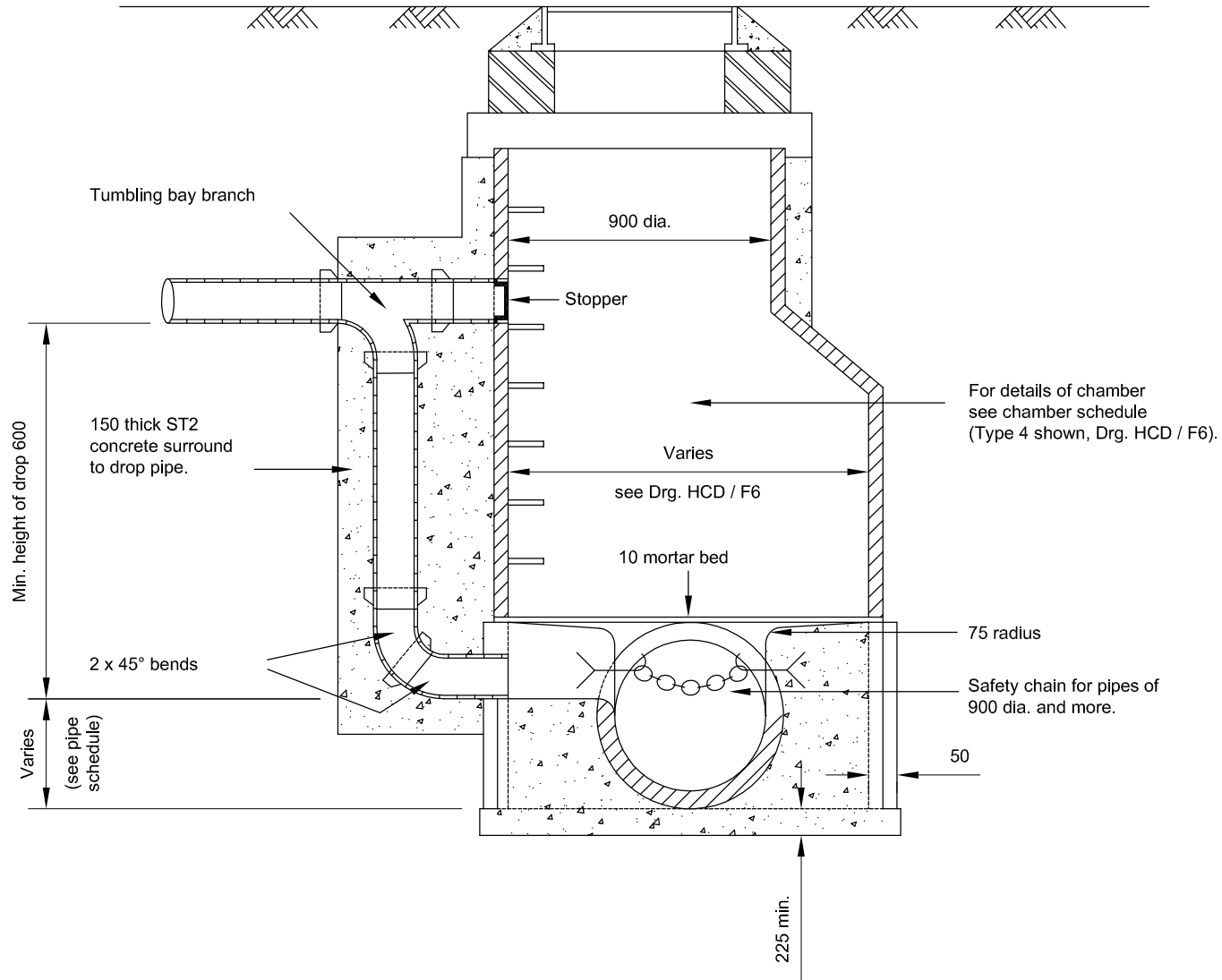
DETAILS OF BACKDROP MANHOLE
